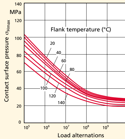
Diagram 12: Contact surface pressure \sigma_{Hmax} , LINNOTAM, grease lubrication
